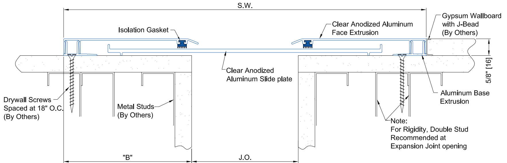
CTR-400 THRU CTR-600 DETAIL WALL-TO-WALL CONDITION
