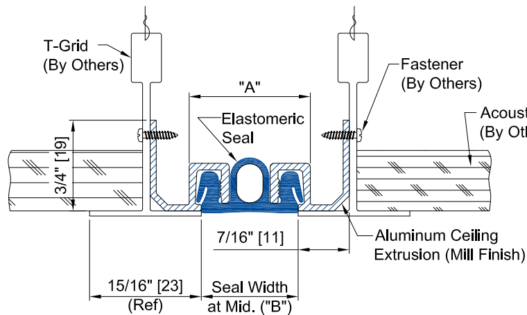
CWCA-100 DETAIL CEILING TO CEILING CONDITION
