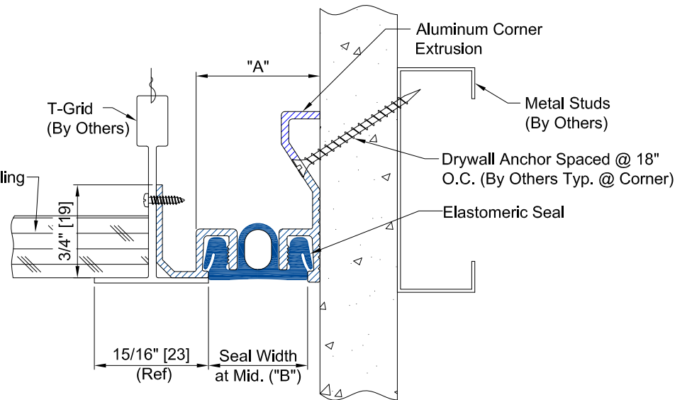
CWCA-100C DETAIL CEILING TO WALL CONDITION
