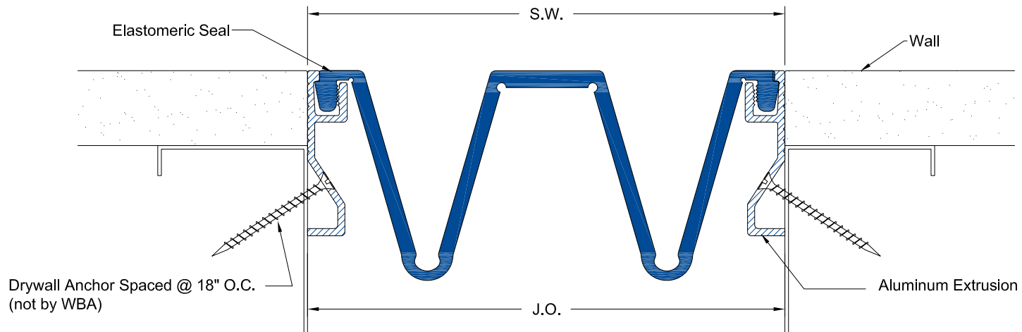
CWWF-400/500/600 typical section wall to wall application gypsum shown - others similar
