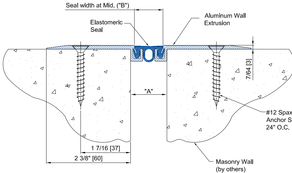
CWWM-100 DETAIL WALL TO WALL CONDITION
