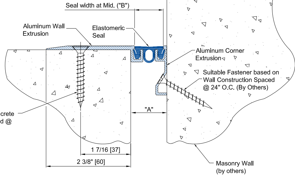
CWWM-100C DETAIL WALL TO WALL CORNER CONDITION
