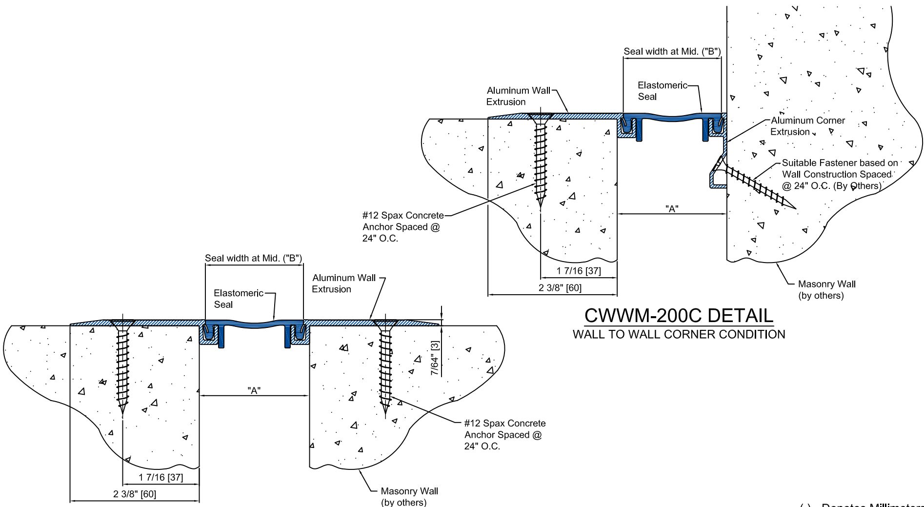
CWWM-200 DETAIL WALL TO WALL CONDITION
