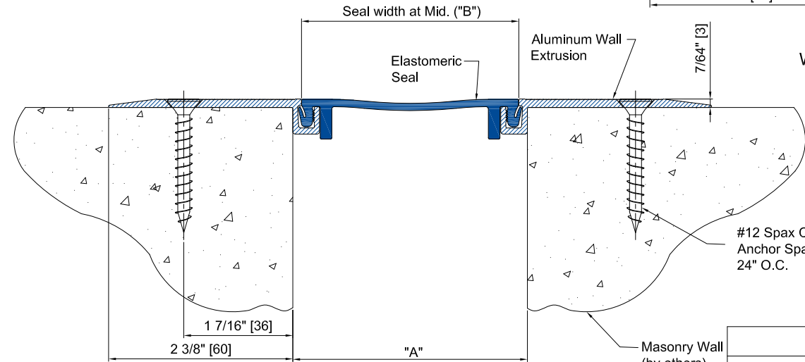
CWWM-300 DETAIL WALL TO WALL CONDITION
