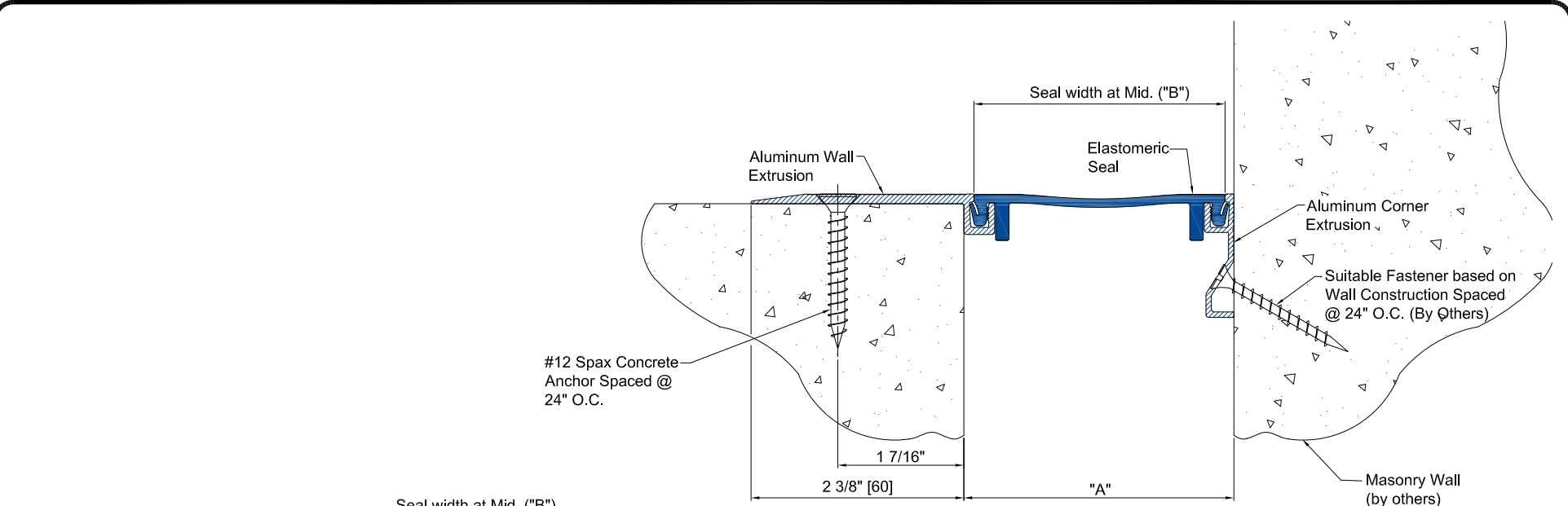
CWWM-300C DETAIL WALL TO WALL CORNER CONDITION
