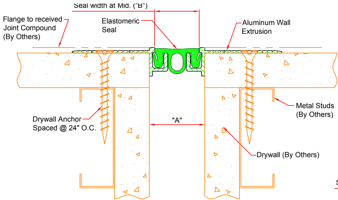
CWWS-100 DETAIL WALL TO WALL CONDITION
