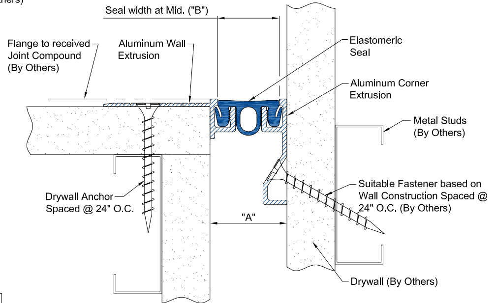
CWWS-100C DETAIL WALL TO WALL CORNER CONDITION
