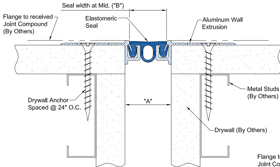
CWWS-100 DETAIL WALL TO WALL CONDITION
