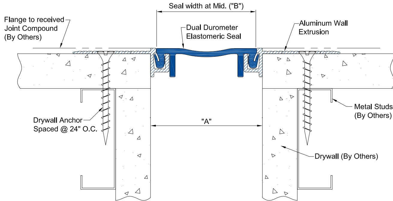
CWWS-200 thru 300 DETAIL WALL TO WALL CONDITION
