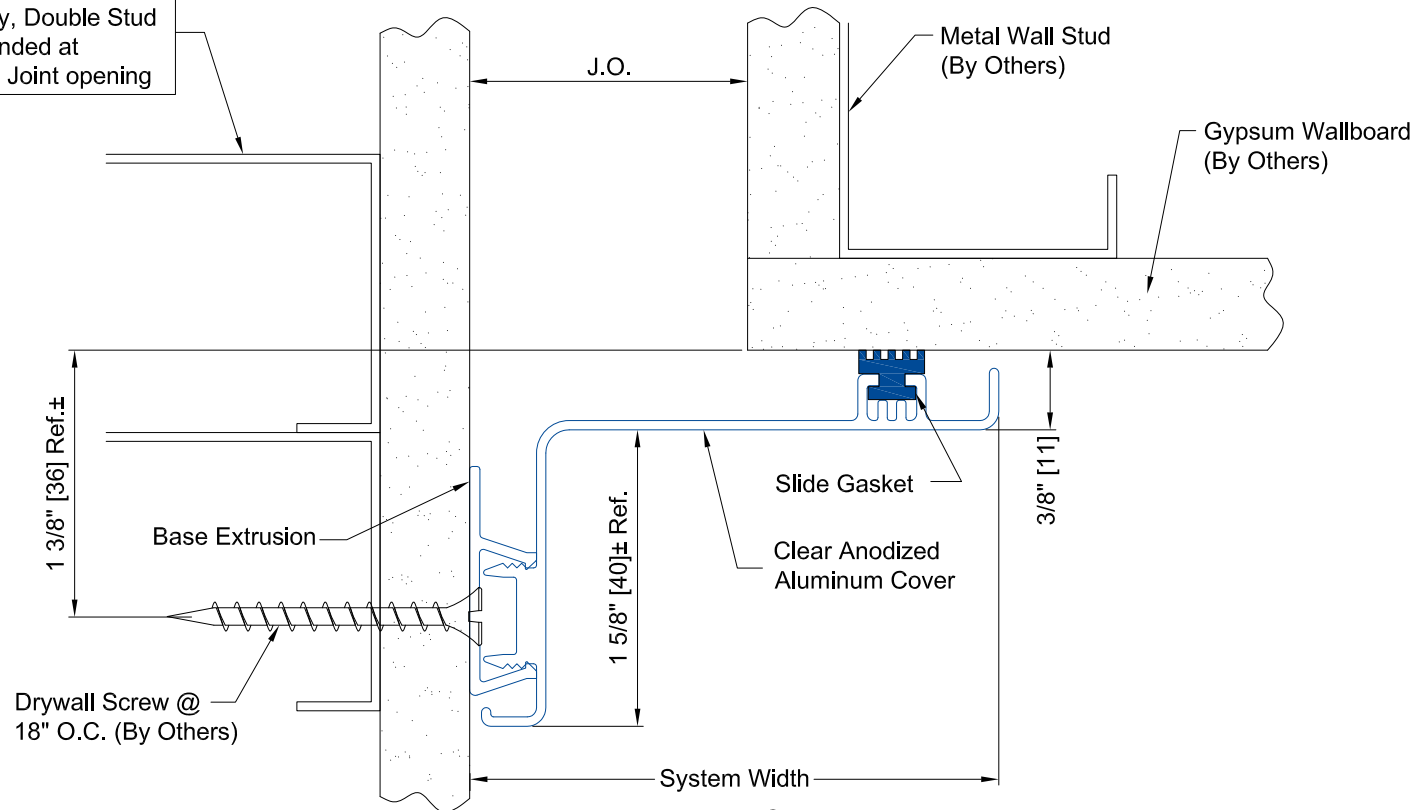
Typical Section Wall to Wall Corner
