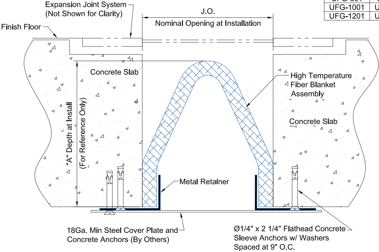
Typical Section UnderSlab Condition
