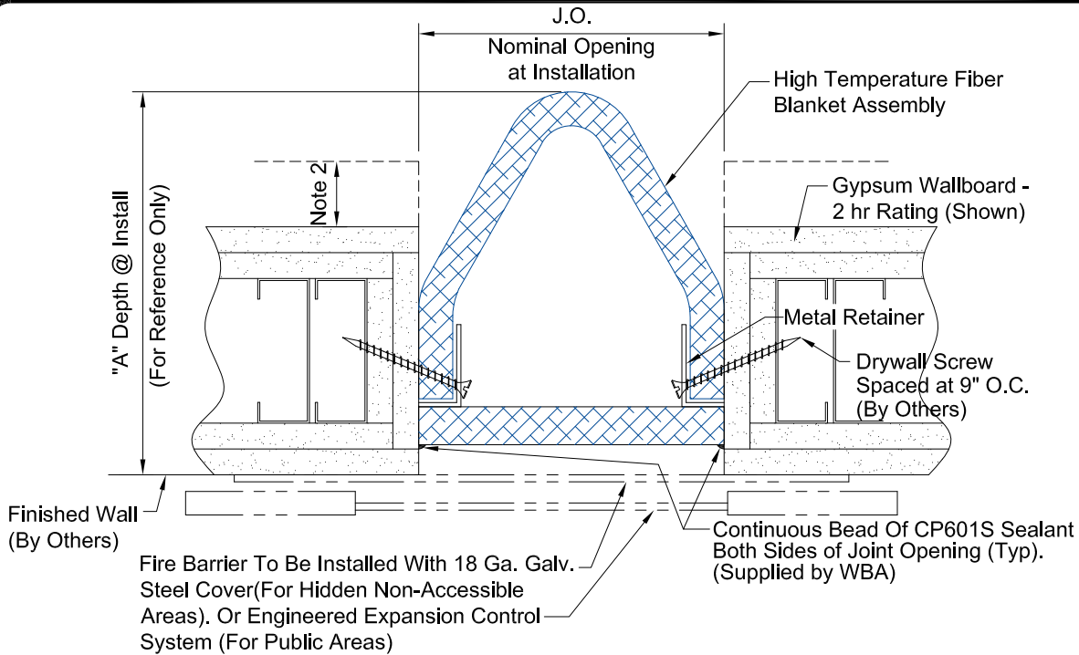
Typical Section 4" thru 26" Flush Condition
