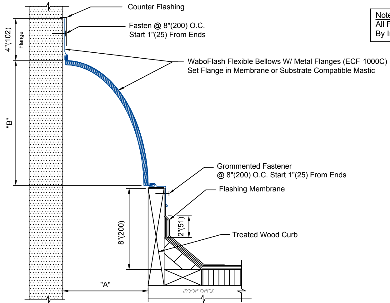
ECF-1000C DETAIL
