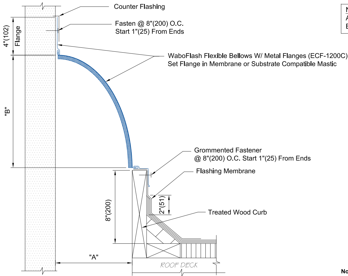
ECF-1200C DETAIL
