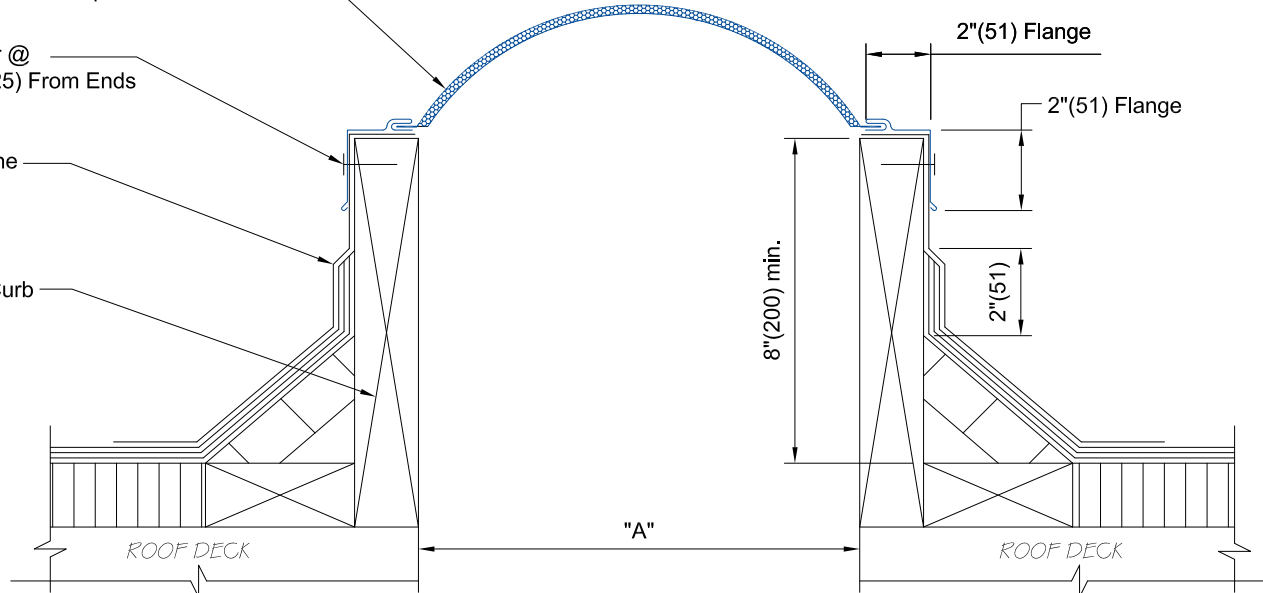
ECF-1200 DETAIL
