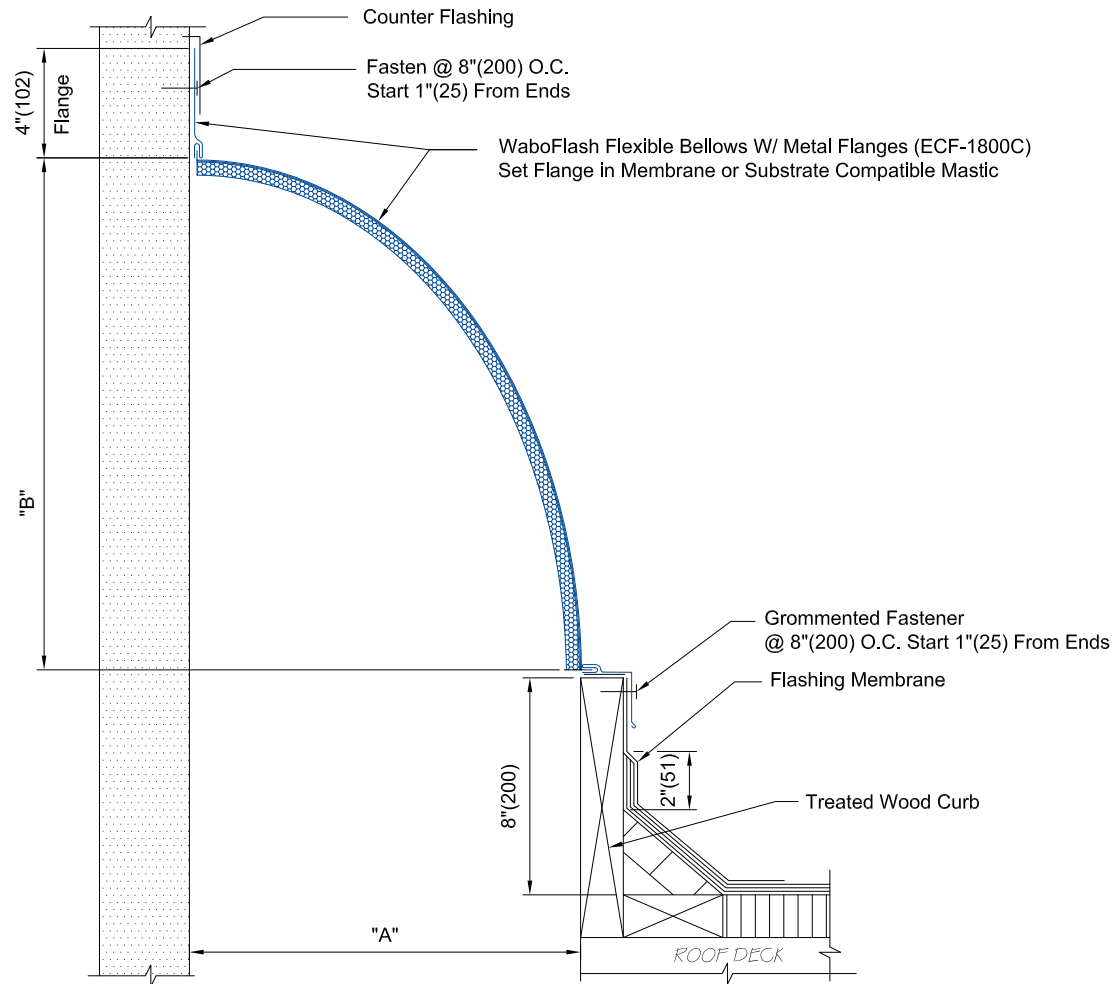
ECF-1800C DETAIL
