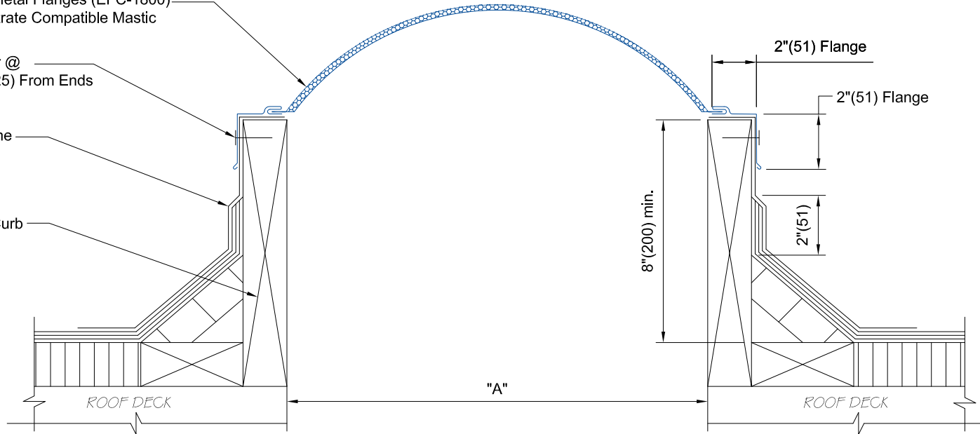
ECF-1800 DETAIL
