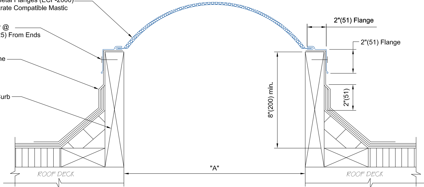
ECF-2000 DETAIL
