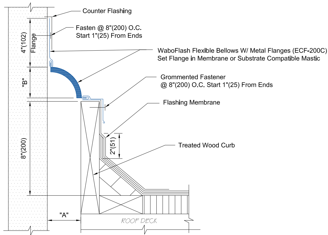
ECF-200C DETAIL
