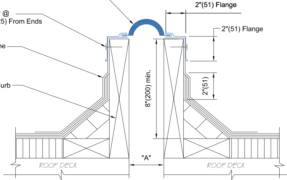
ECF-200 DETAIL
