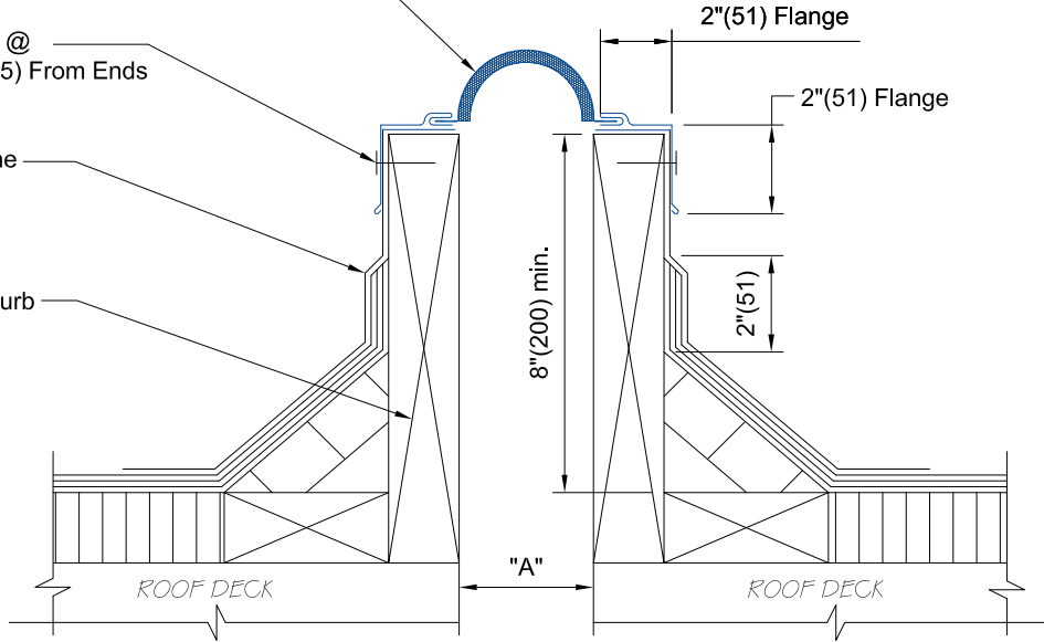
ECF-300 DETAIL
