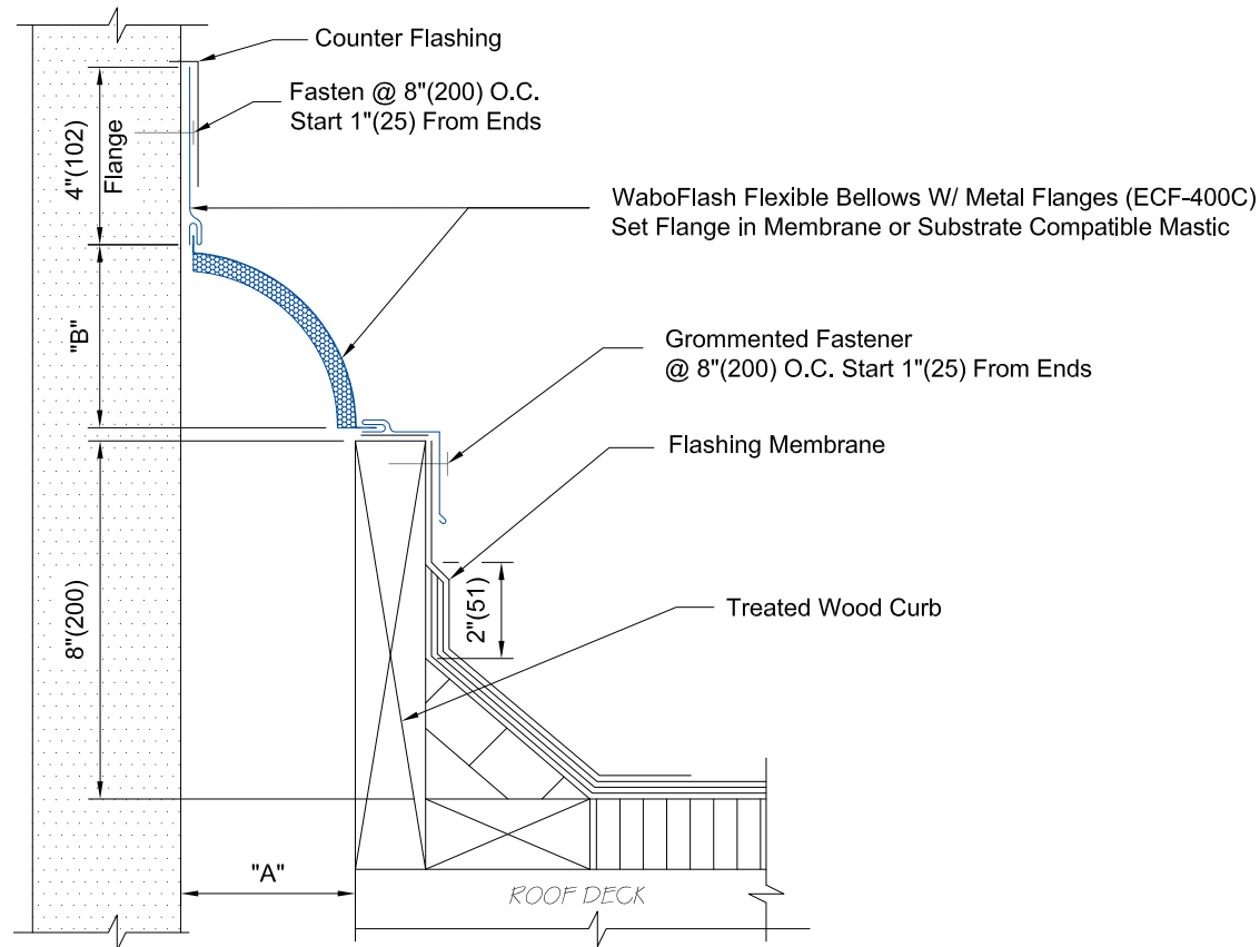
ECF-400C DETAIL
