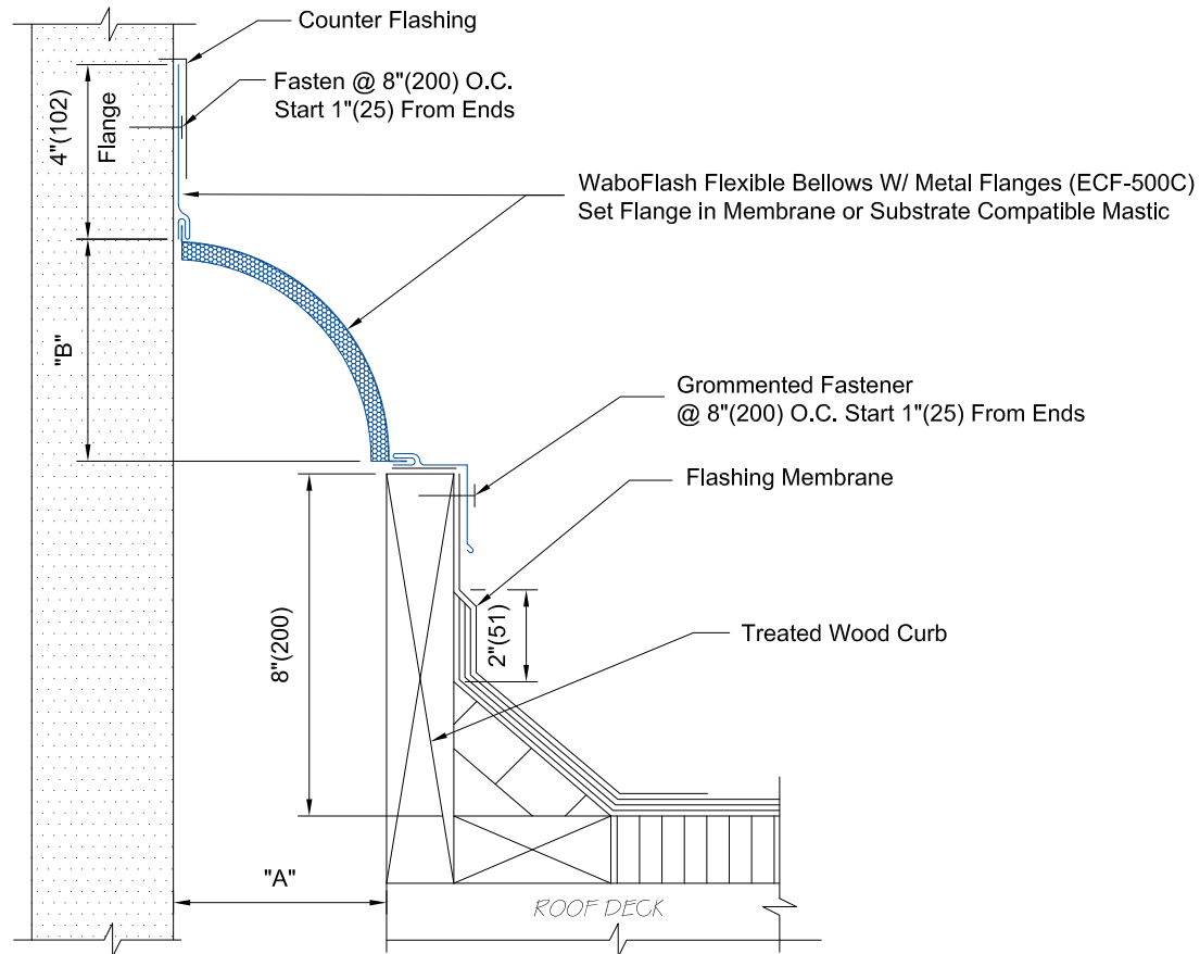
ECF-500C DETAIL
