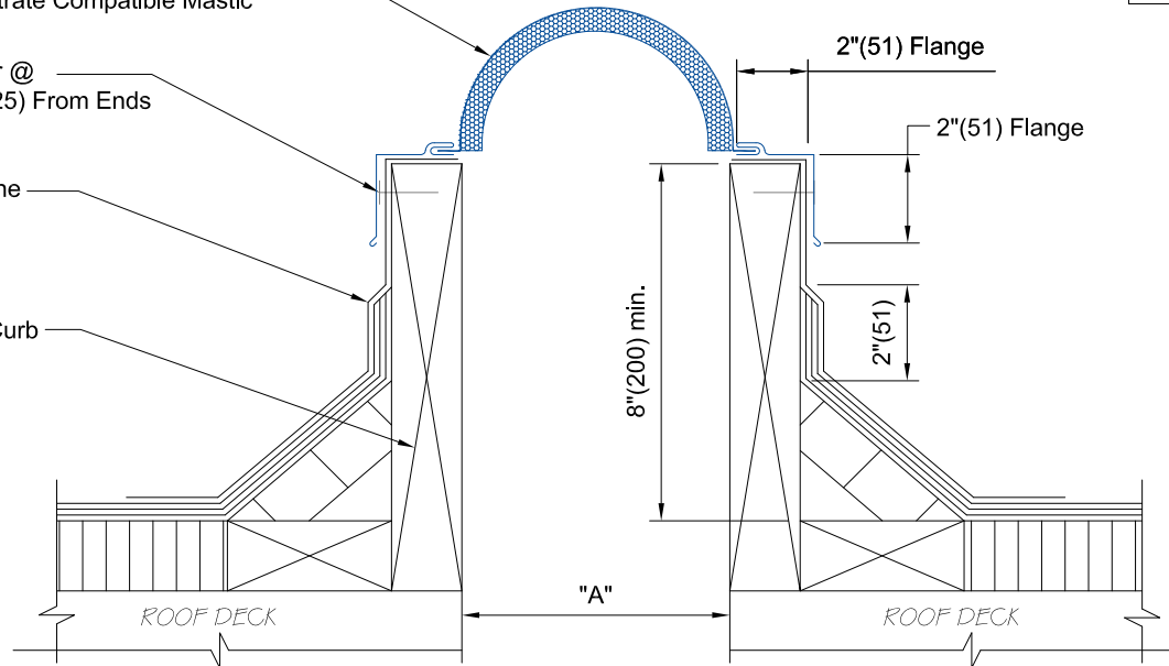
ECF-600 DETAIL
