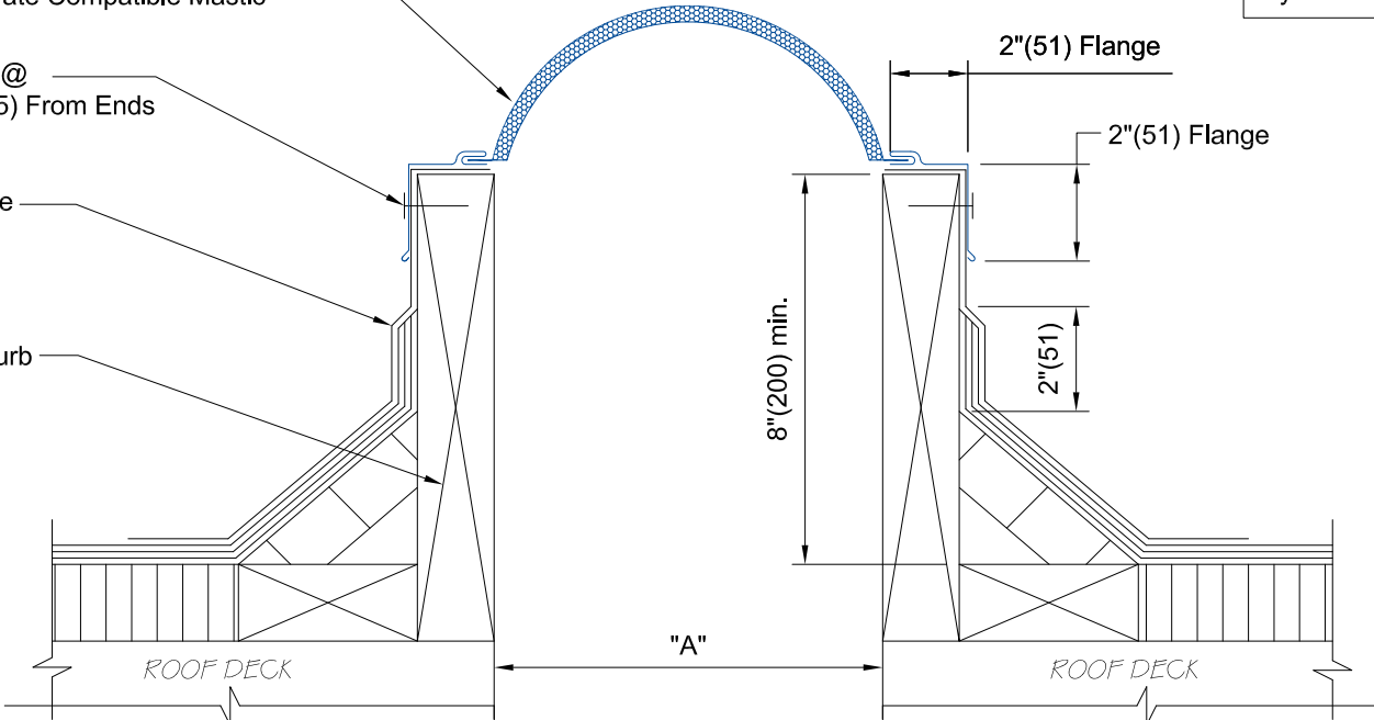
ECF-800 DETAIL
