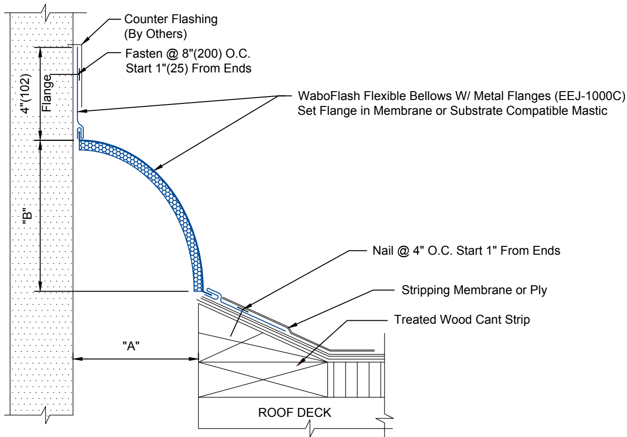
EEJ-1000C DETAIL
