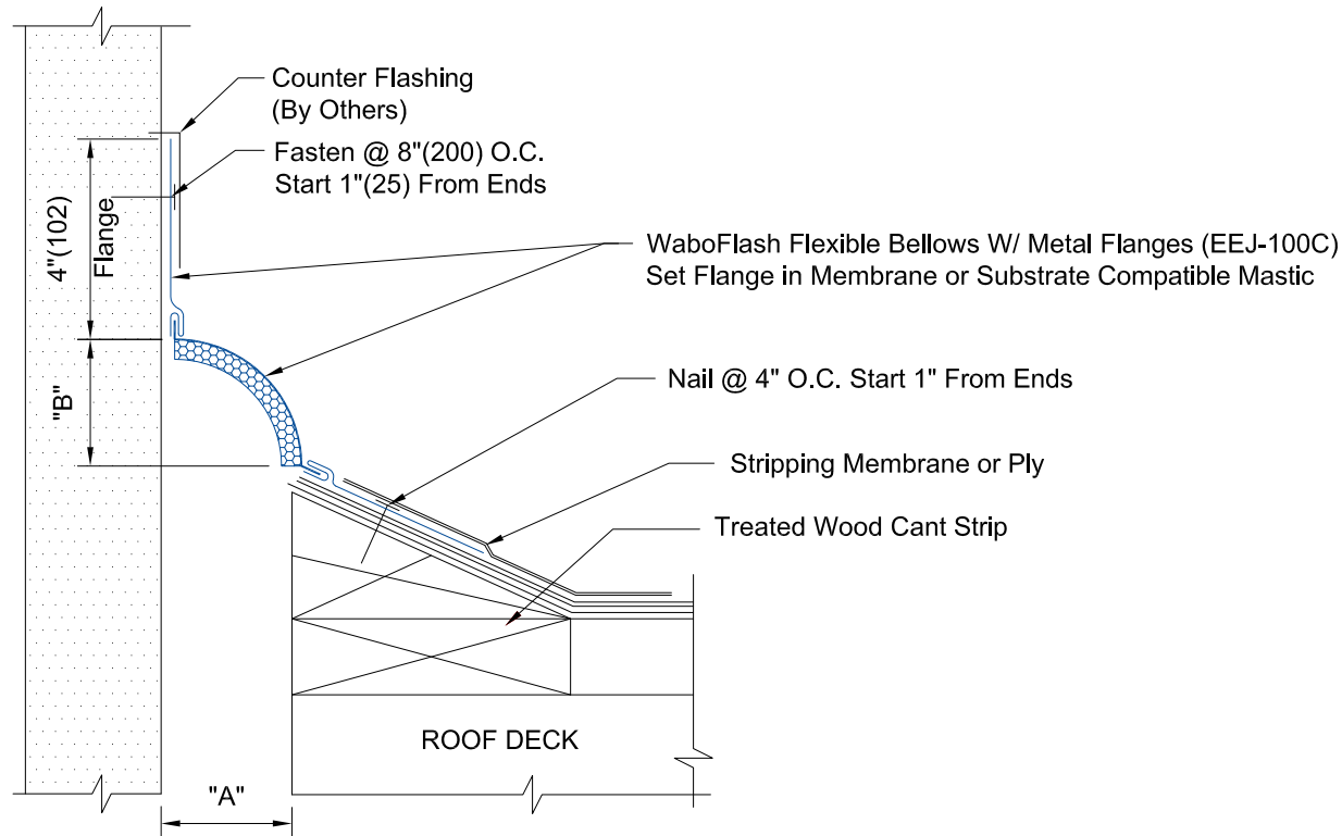
EEJ-100C DETAIL
