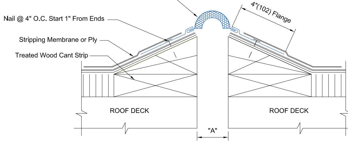
EEJ-100 DETAIL
