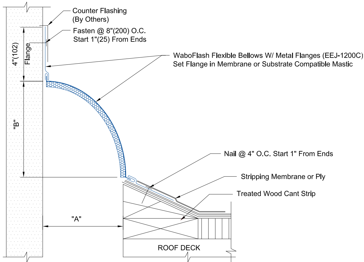
EEJ-1200C DETAIL
