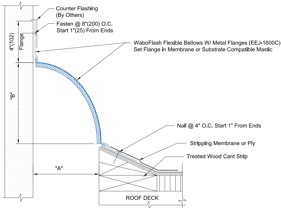
EEJ-1600C DETAIL
