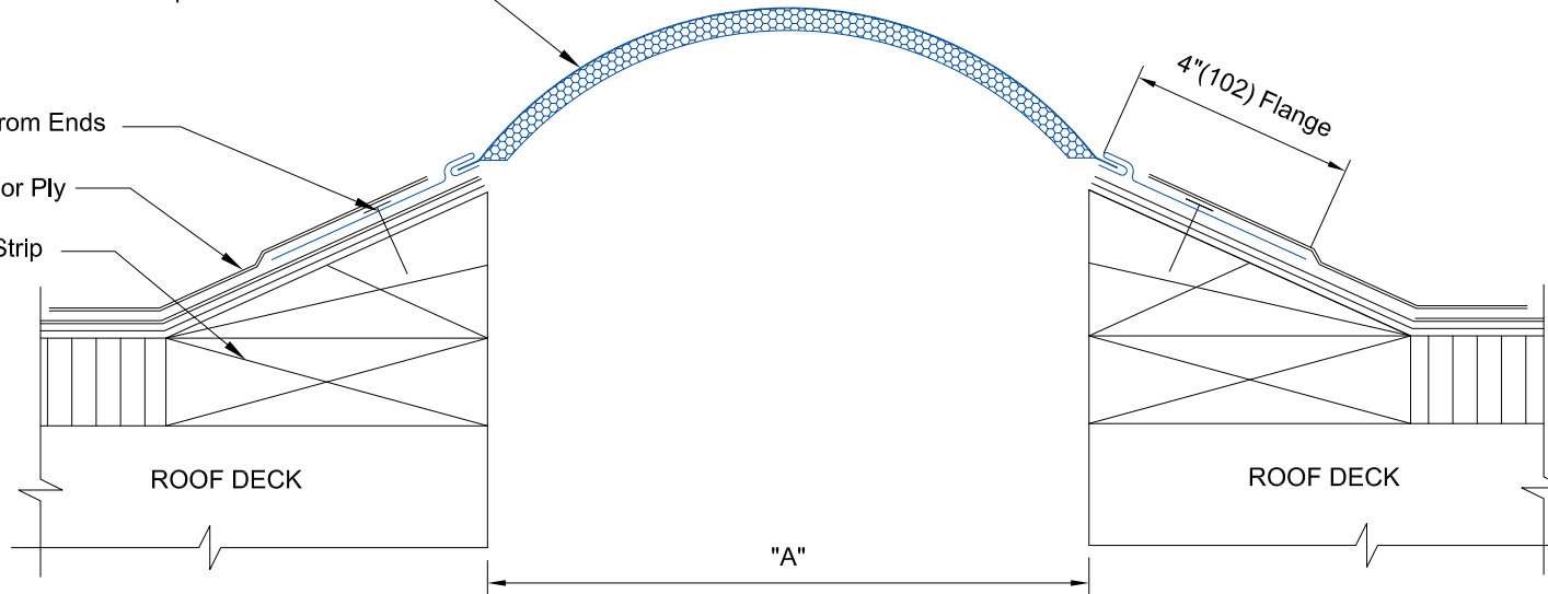
EEJ-1600 DETAIL
