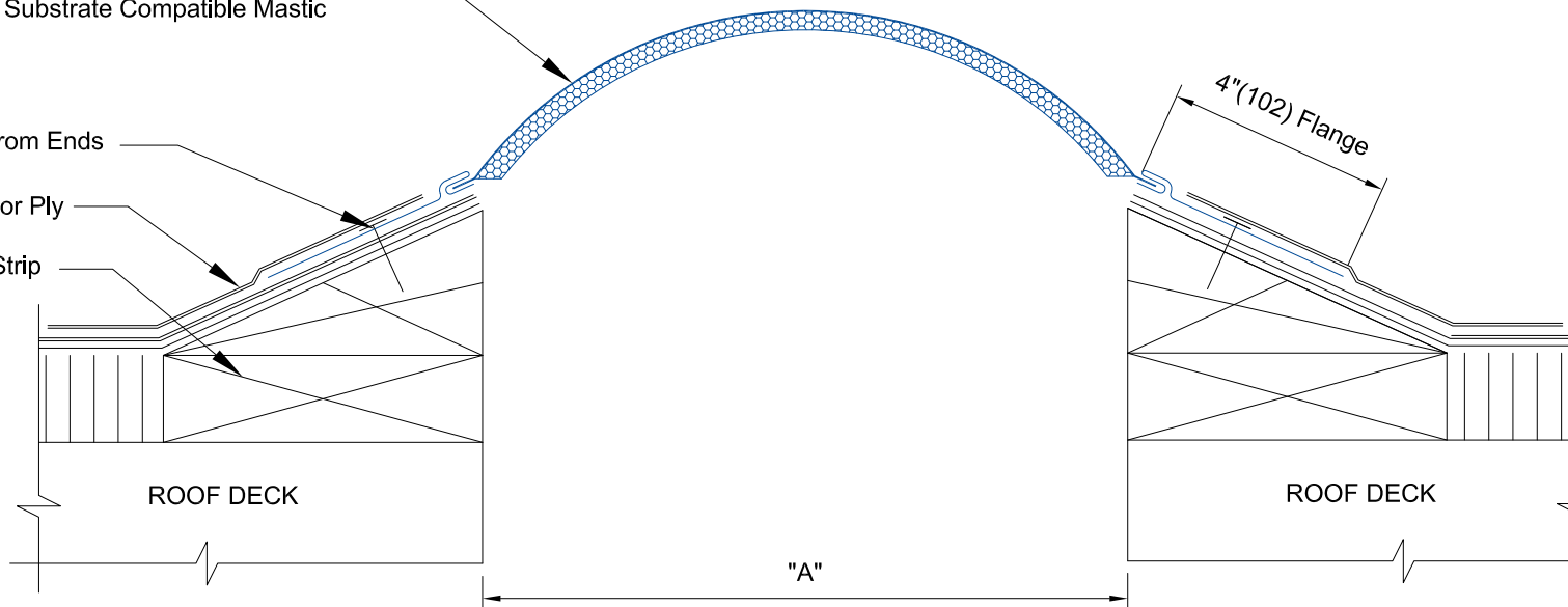
EEJ-2000 DETAIL
