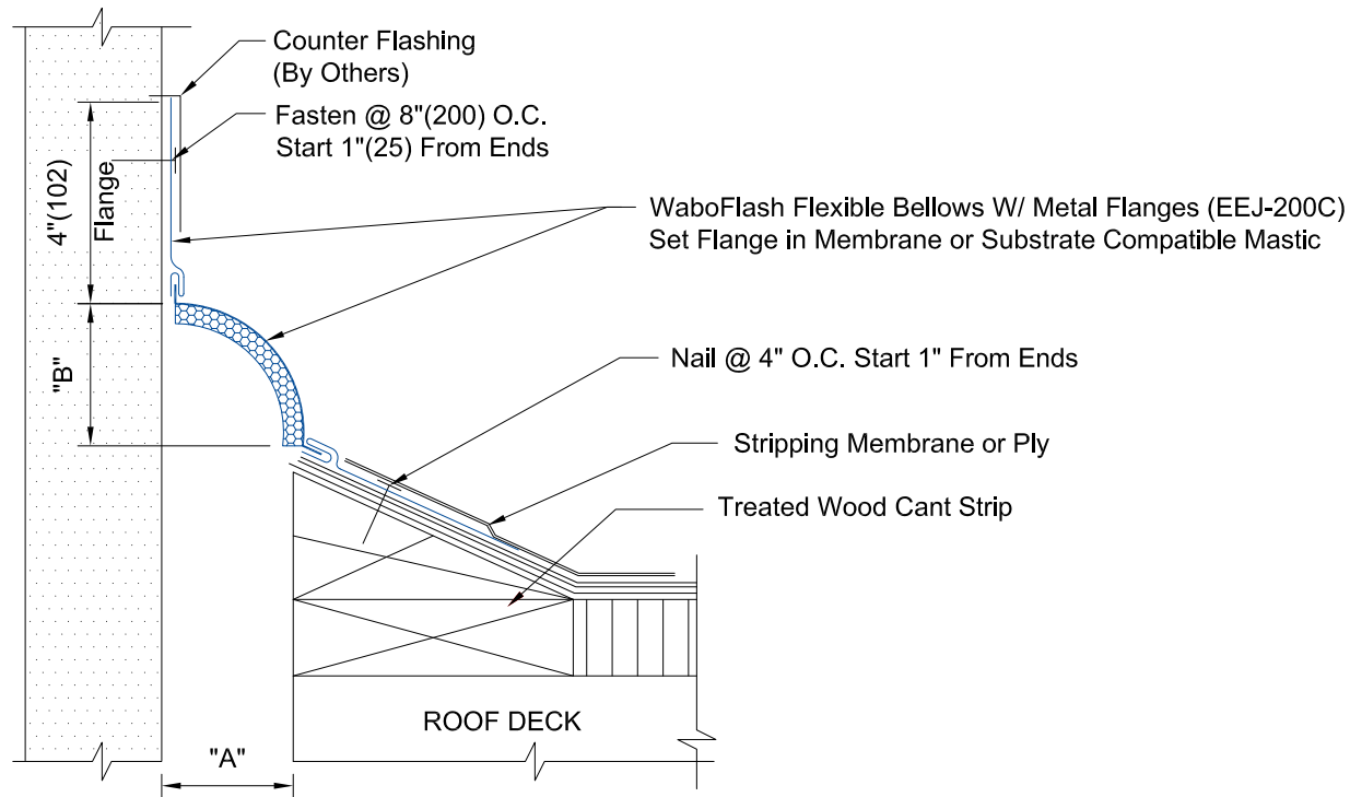
EEJ-200C DETAIL
