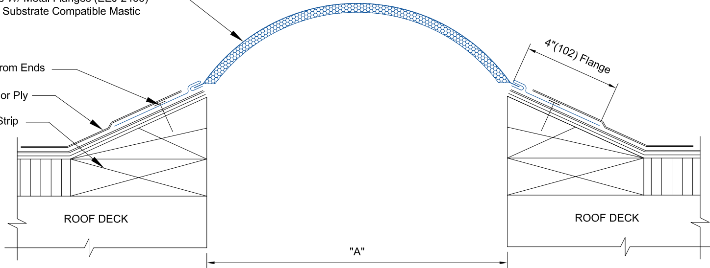
EEJ-2400 DETAIL
