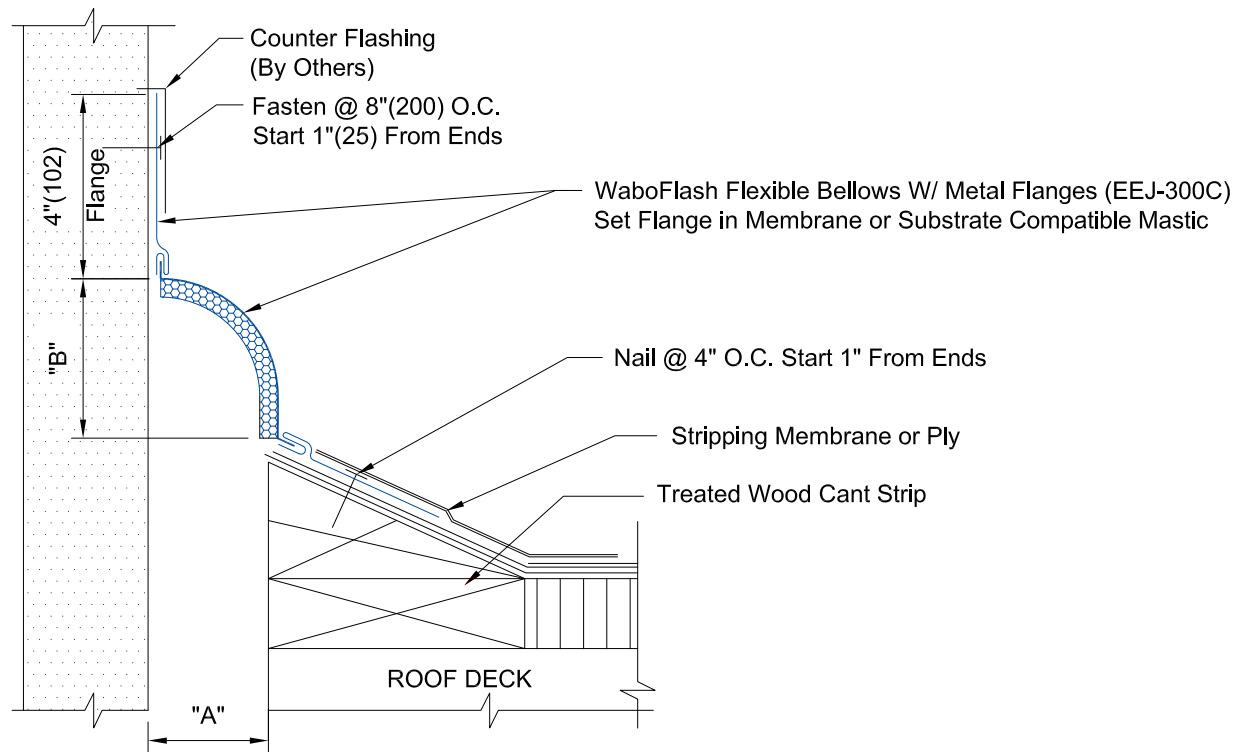
EEJ-300C DETAIL
