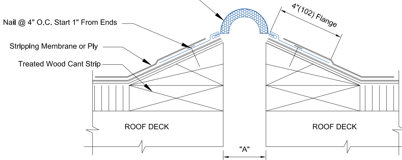
EEJ-300 DETAIL
