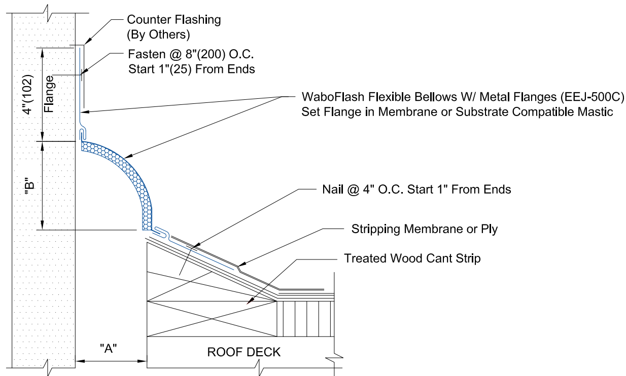
EEJ-500C DETAIL
