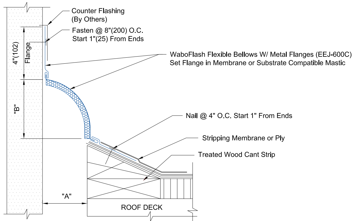
EEJ-600C DETAIL
