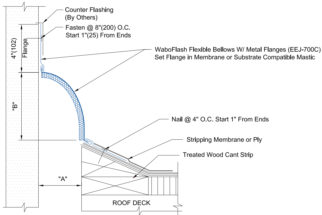
EEJ-700C DETAIL
