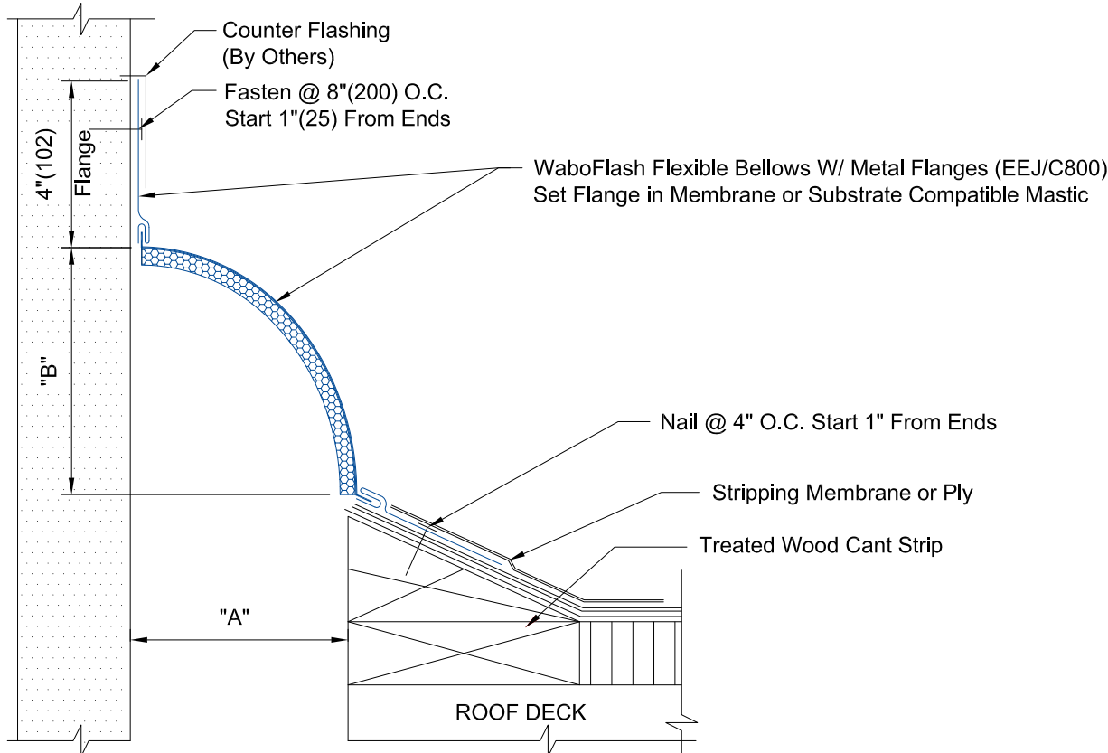
EEJ-800C DETAIL
