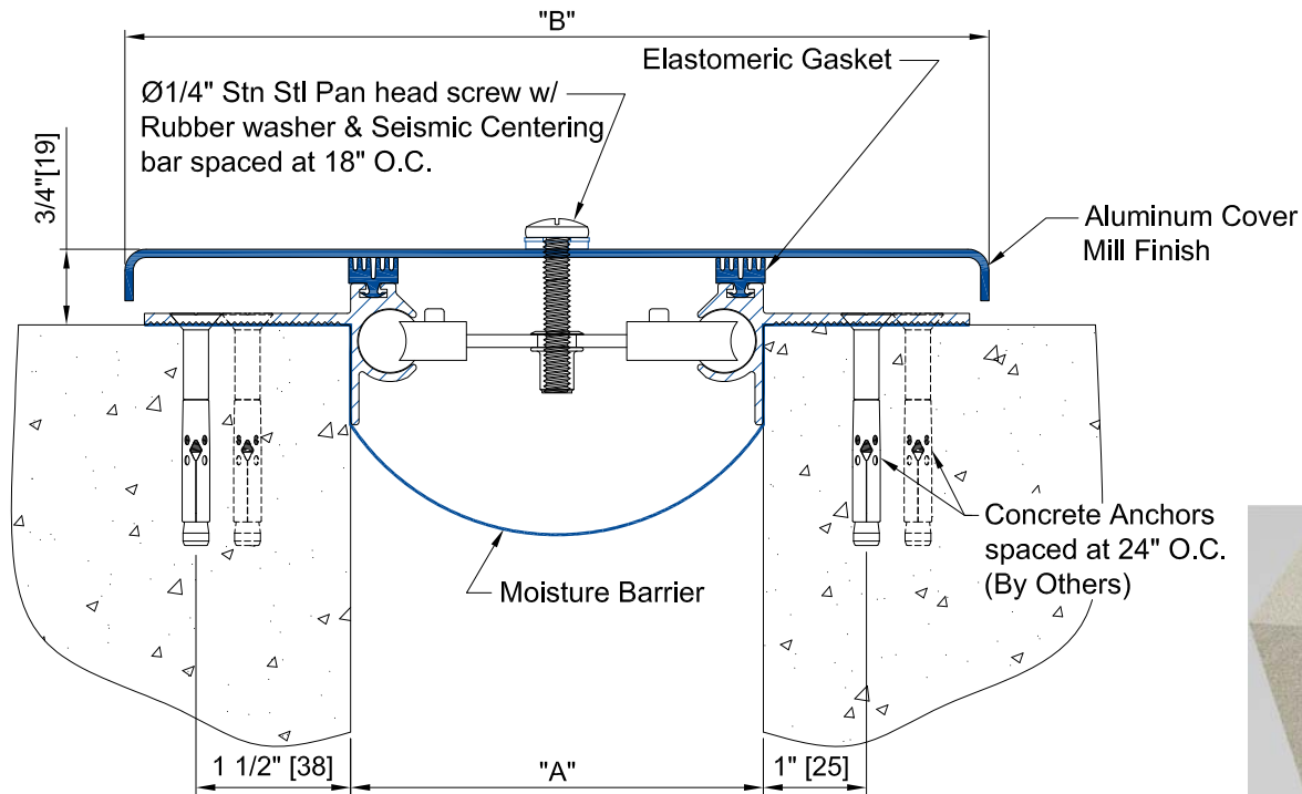
WFE-200 THRU WFE-2400 DETAIL WALL-TO-WALL EXTERIOR CONDITION NOT TO SCALE
