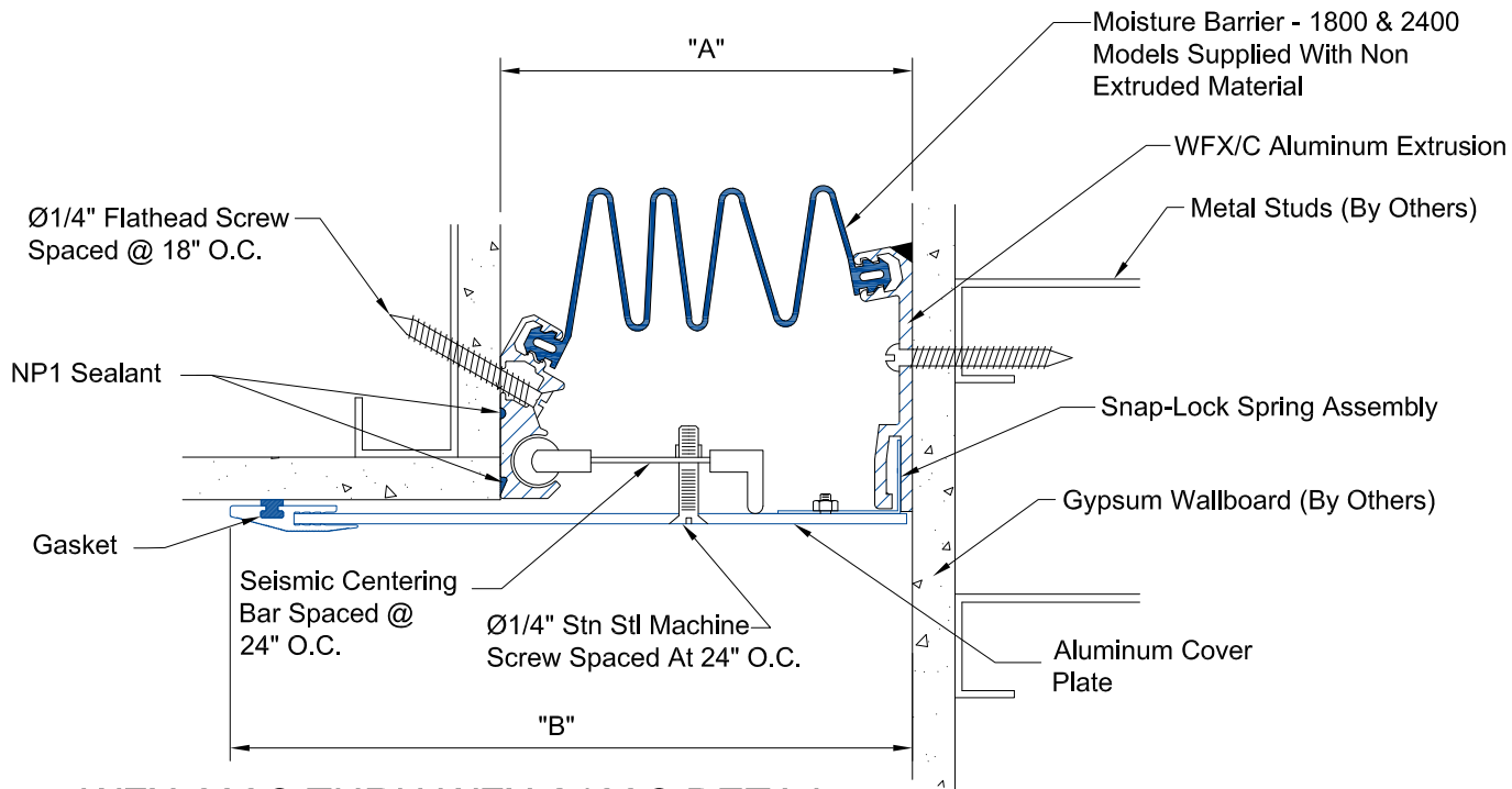
WFX-600C THRU WFX-2400C DETAIL WALL-TO-WALL EXTERIOR CORNER CONDITION
