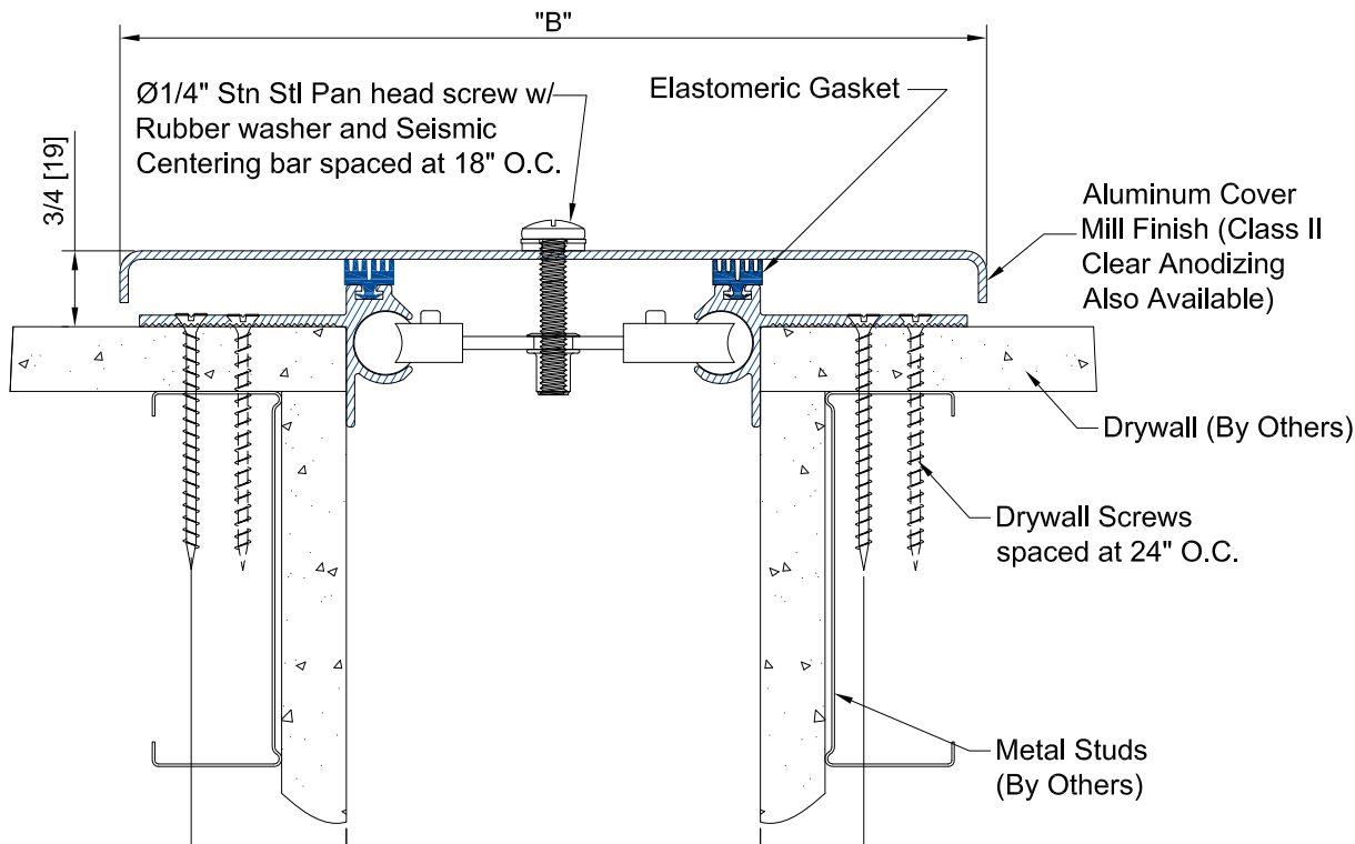
WFI-200 Thru WFI-2400 DETAIL WALL-TO-WALL INTERIOR CONDITION
