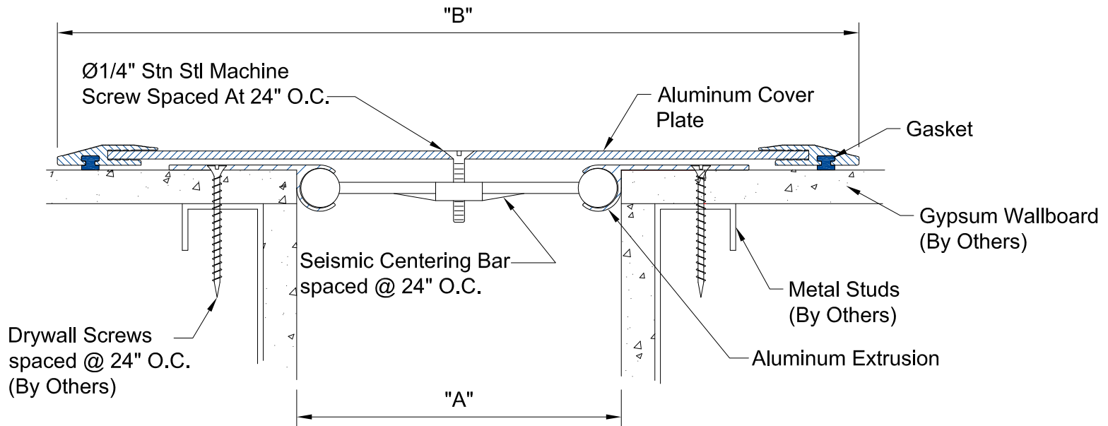
WFT-400 THRU WFT-2400 DETAIL WALL-TO-WALL INTERIOR CONDITION
