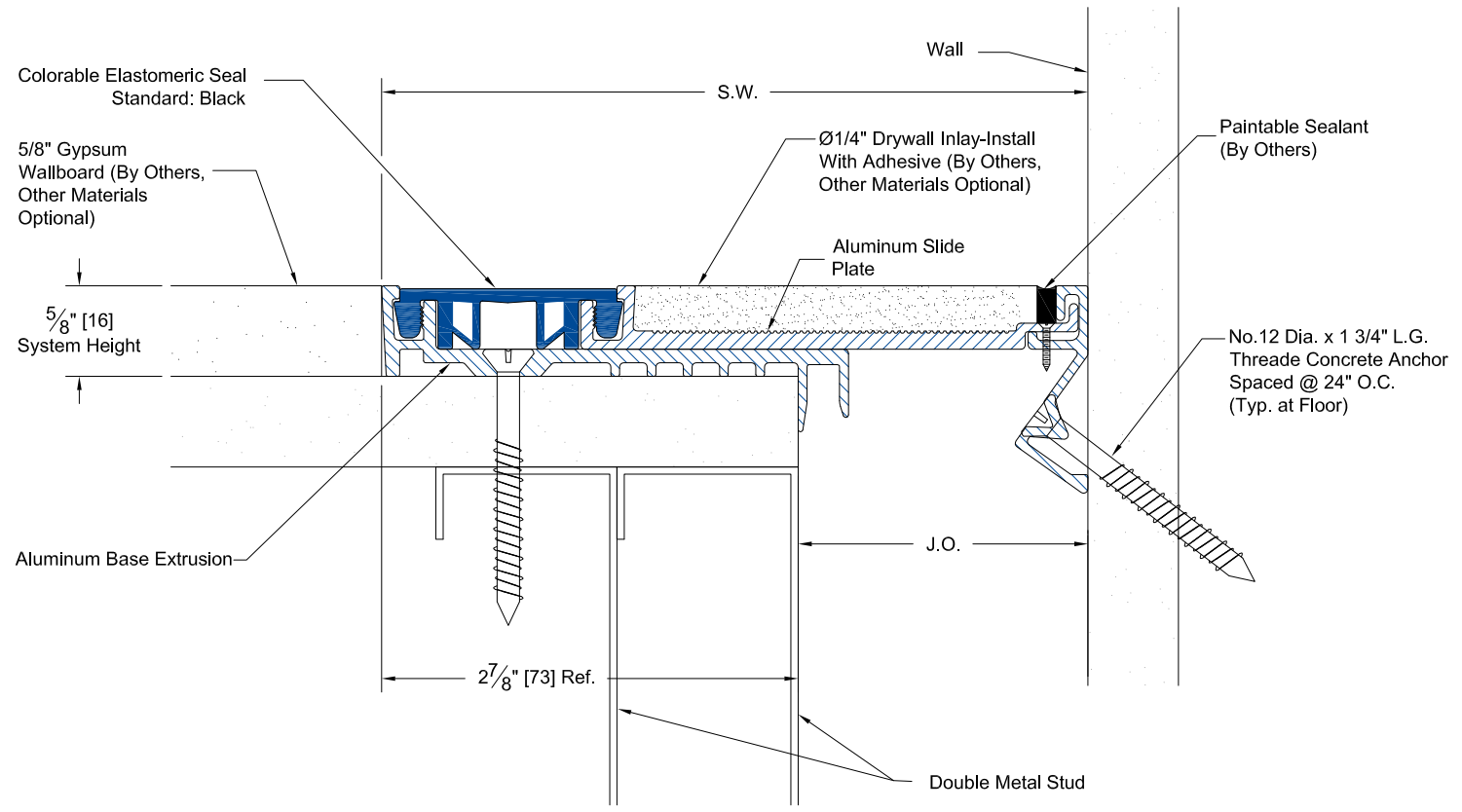
Typical Section
