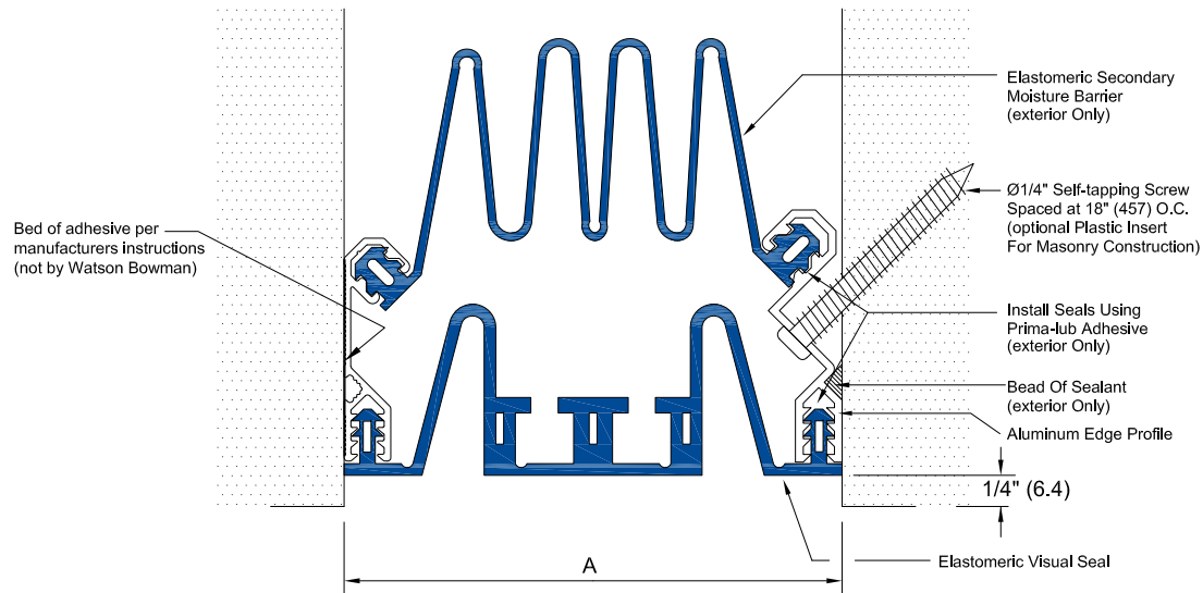
WSC-400 DETAIL
