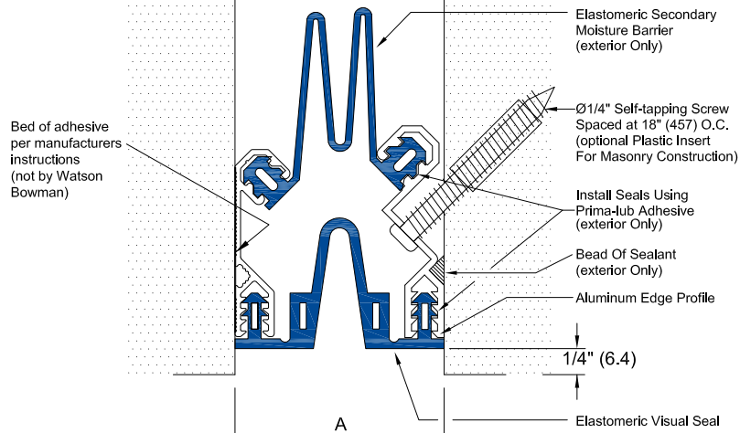
WSC-200 DETAIL
