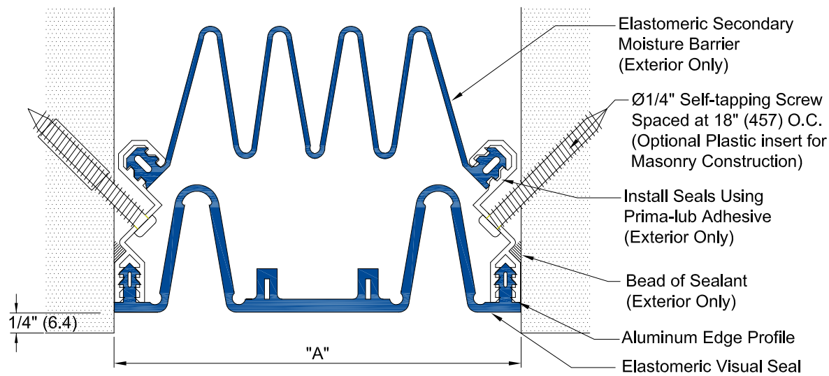
WSW-500 DETAIL
